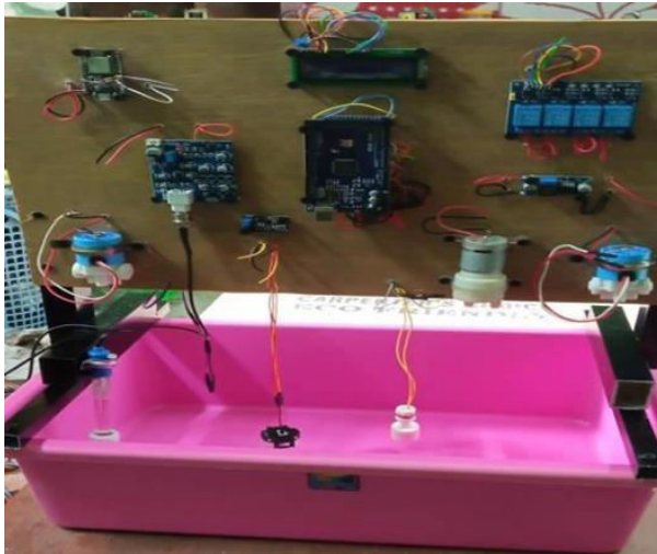
Fig.2.Hardware implementation
