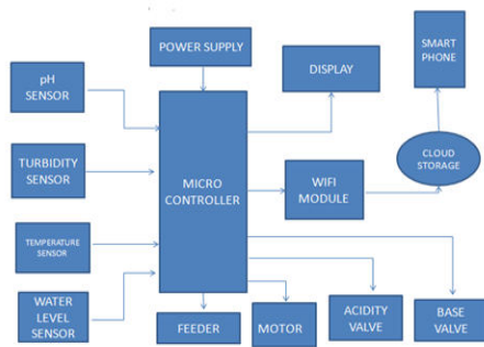
Fig.1 System Architecture
